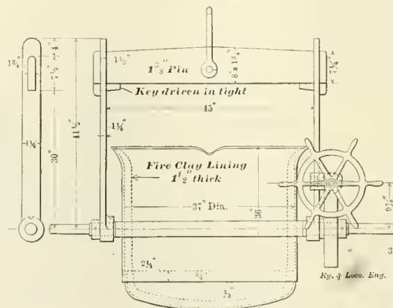
EASILY MADE FOUNDRY SHOP LADLE.
